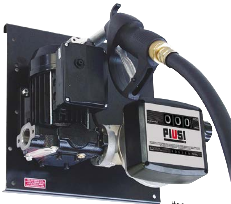
Hose: - length 4 m - Ø 3/4"
